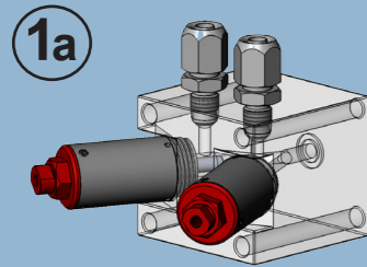
Emulsion block - without recirculation
