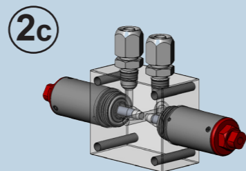
Intermediate block threaded - without recirculation
