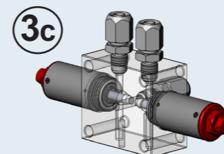
Output block - with controlled recirculation
