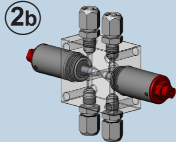
Intermediate block - with recirculation
