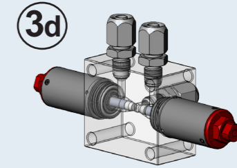
Blind output block - without recirculation
