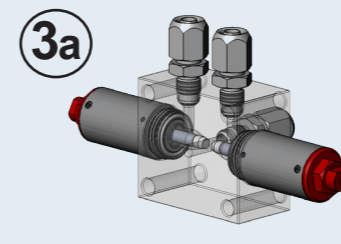
Output block - without recirculation
