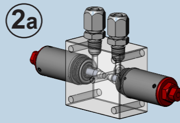
Intermediate block - without recirculation
