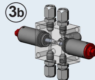
Output block - with recirculation
