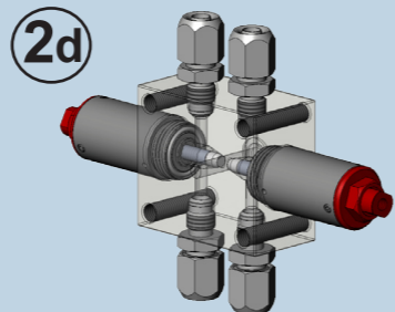
Intermediate block threaded - with recirculation
