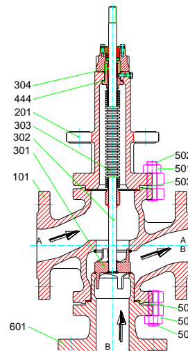
MV 5324, PV 6324 DN 20 – 150, PN 16 – 25
