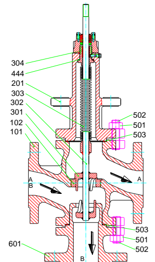
MV 5334, PV 6334 DN 20 – 150, PN 16 – 25
