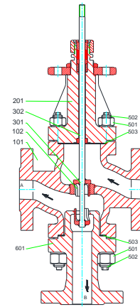
MV 5331, PV 6331 DN 25 – 50, PN 63 – 100
